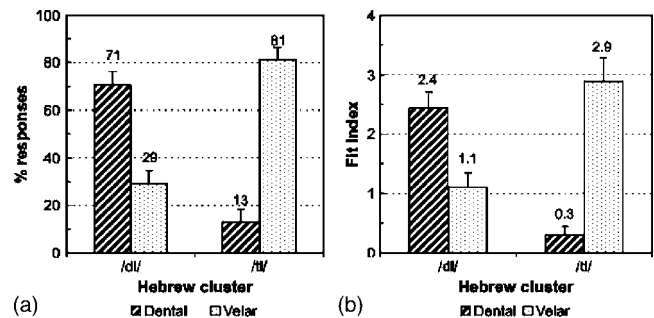
FIG. 2. Categorization of the initial stop of Hebrew /dl/ and /tl/ by French subjects: (a) Percentages of dental and velar responses, and (b) corresponding “fit indexes.” Error bars indicate standard error.
